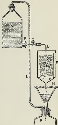
FIG. 27.—Andrès' Filtering Apparatus.
